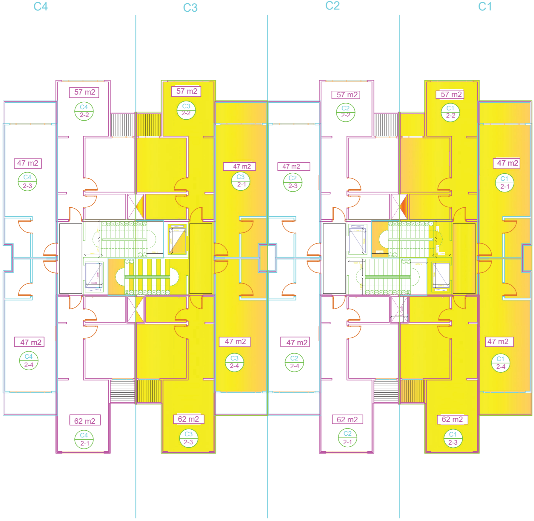
TYPICAL.FL
